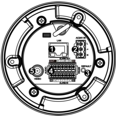
Connectors
